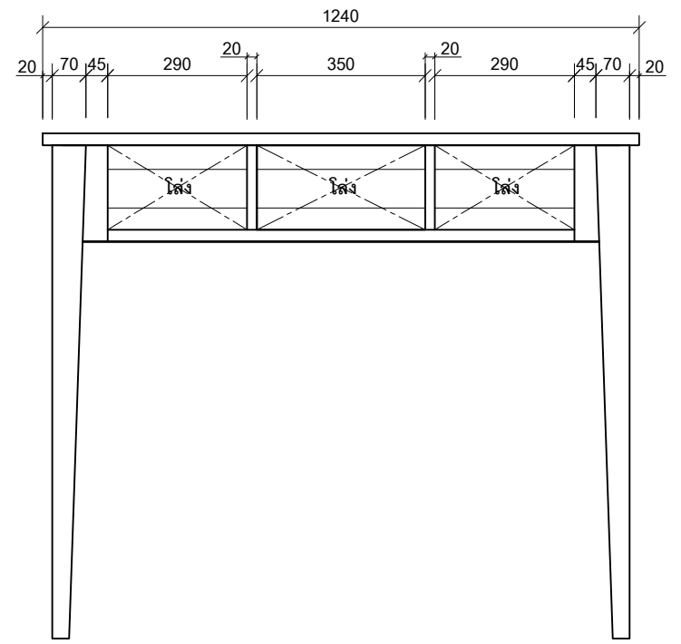
BACK SCALE 1:10
