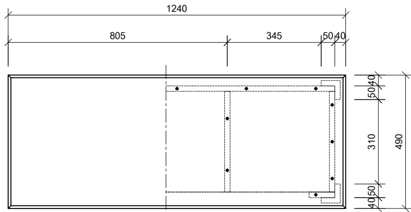
TOP SCALE 1:10
